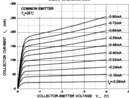
Static Characteristic
