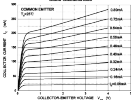
Static Characteristic
